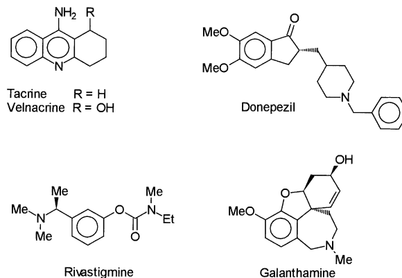
Figure 1. Structural formulas for AChEI.
