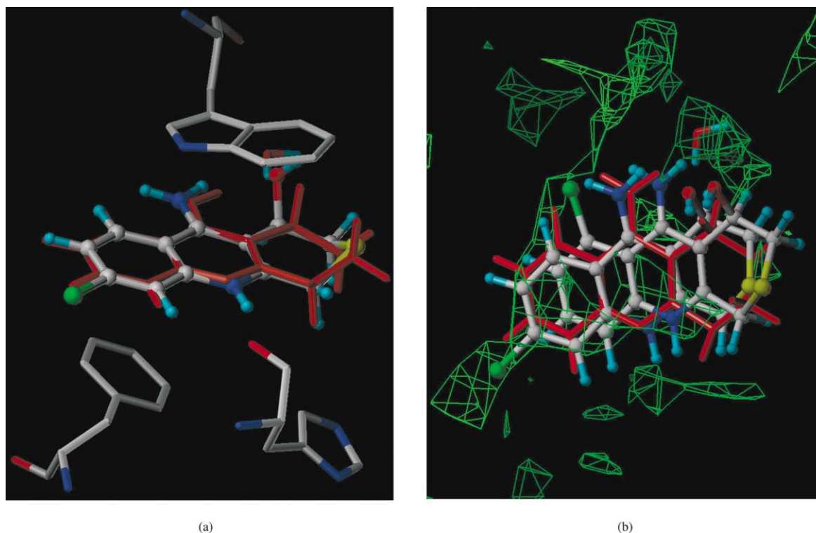
Figure 3. (a) Structure of 6-chlorothiopyranoquinoline 5eg superimposed to tacrine; (b) GRID maps of the interaction between the enzyme and chlorine atom probes shown for compounds 5cg , 5eg , and tacrine.
