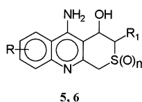
Figure 2. Thiopyranoquinolines prepared in this study (for R, R 1 and n, see Scheme 1).
