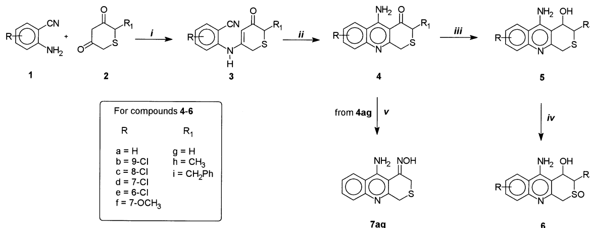
Scheme 1. Reagents: (i) dry benzene, TsOH, reflux; (ii) K 2 CO 3 , CuCl, DMF, 90 °C; (iii) LiAlH 4 , dry THF; (iv) 50% MCPBA, MeOH; (v) NH 2 OH, pyridine, EtOH.
